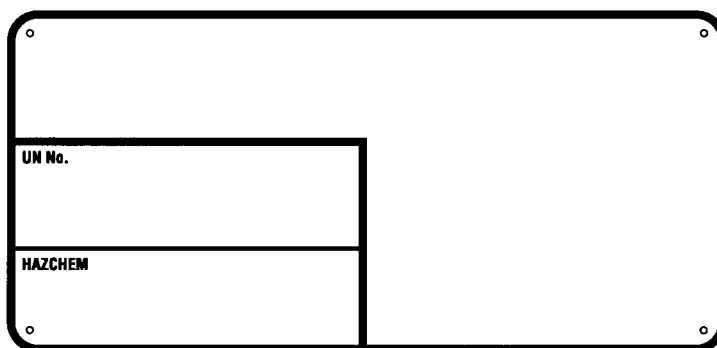
figure 3—form and dimensions of emergency information sign for single class of hazardous substance
